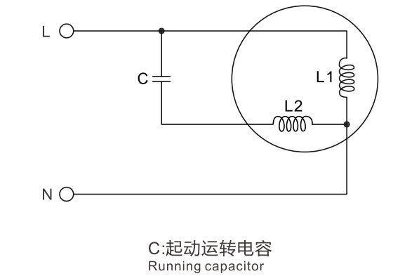
典型线路图 Typical circuit
