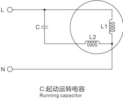
典型线路图 Typical circuit
