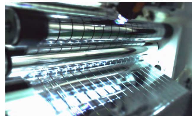
薄膜分切机 Film splitter
